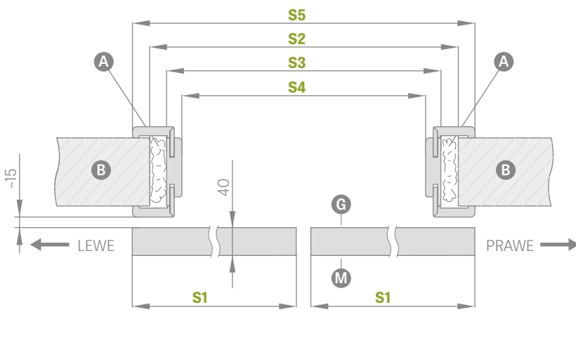
WALL-MOUNTED SLIDING DOOR SYSTEM WITH DOOR OPENING HOUSING
